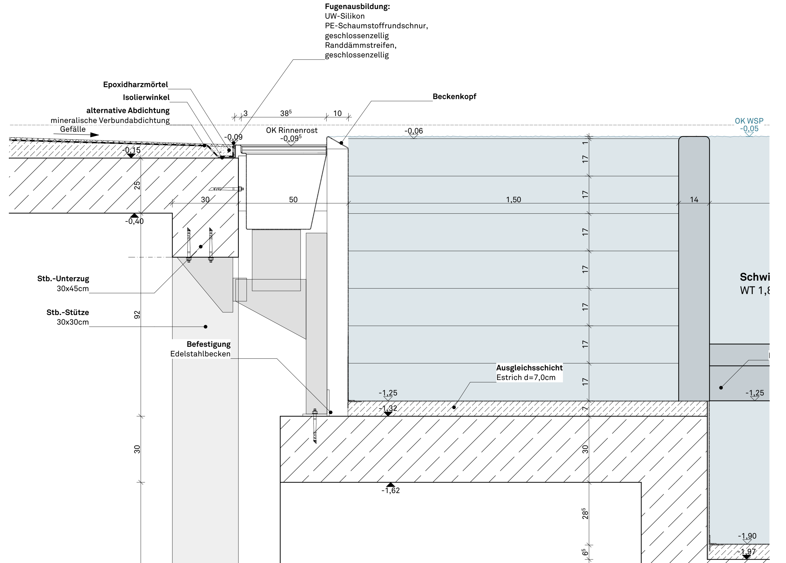
DETAIL 1:10 SB Beckentreppe WT 1,80m
