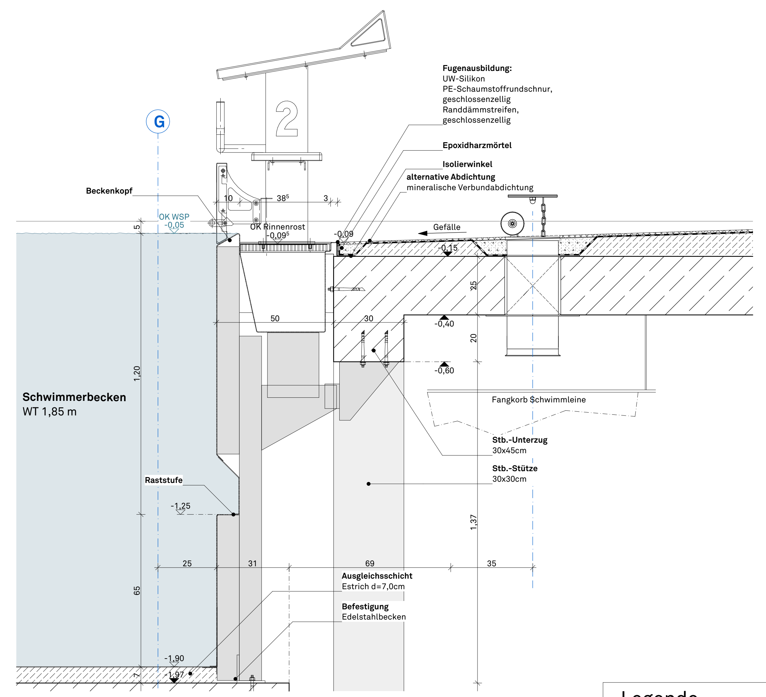
DETAIL 1:10 SB Startblock WT 1,80m
