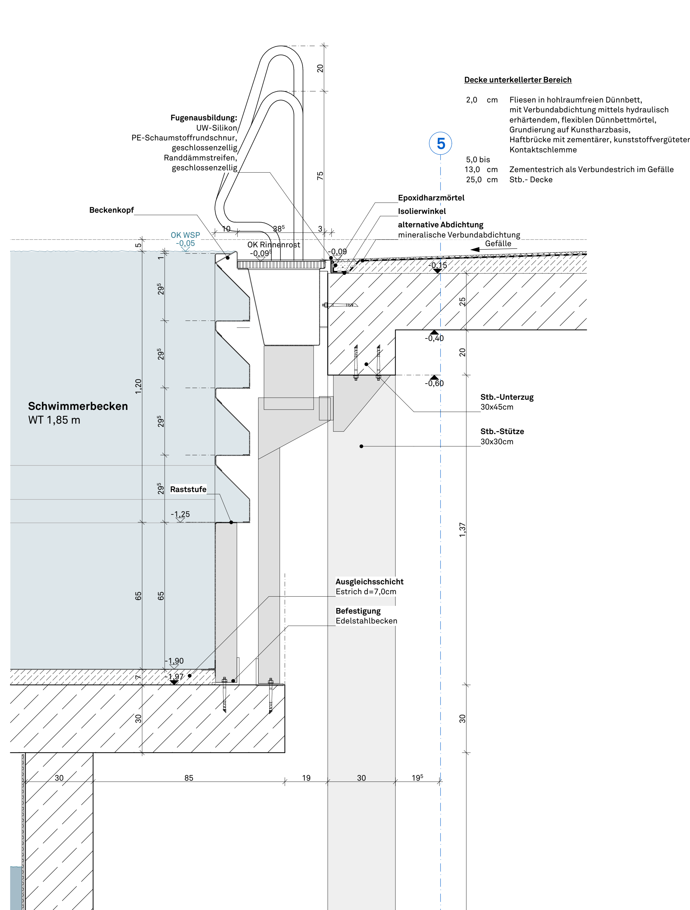
DETAIL 1:10 SB Beckenleiter WT 1,80m
