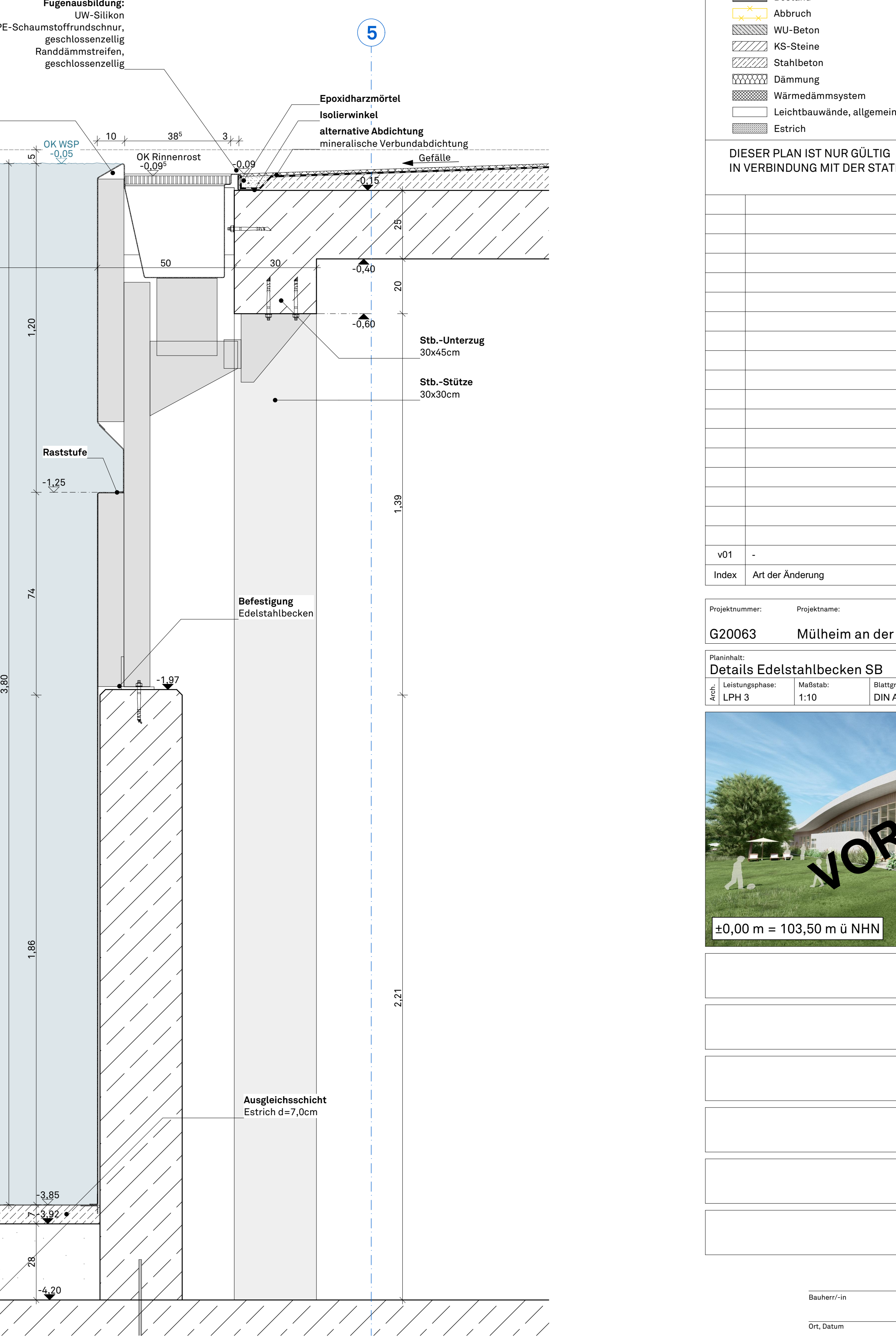
DETAIL 1:10 SB Beckenkopf / Wand WT 3,80m
